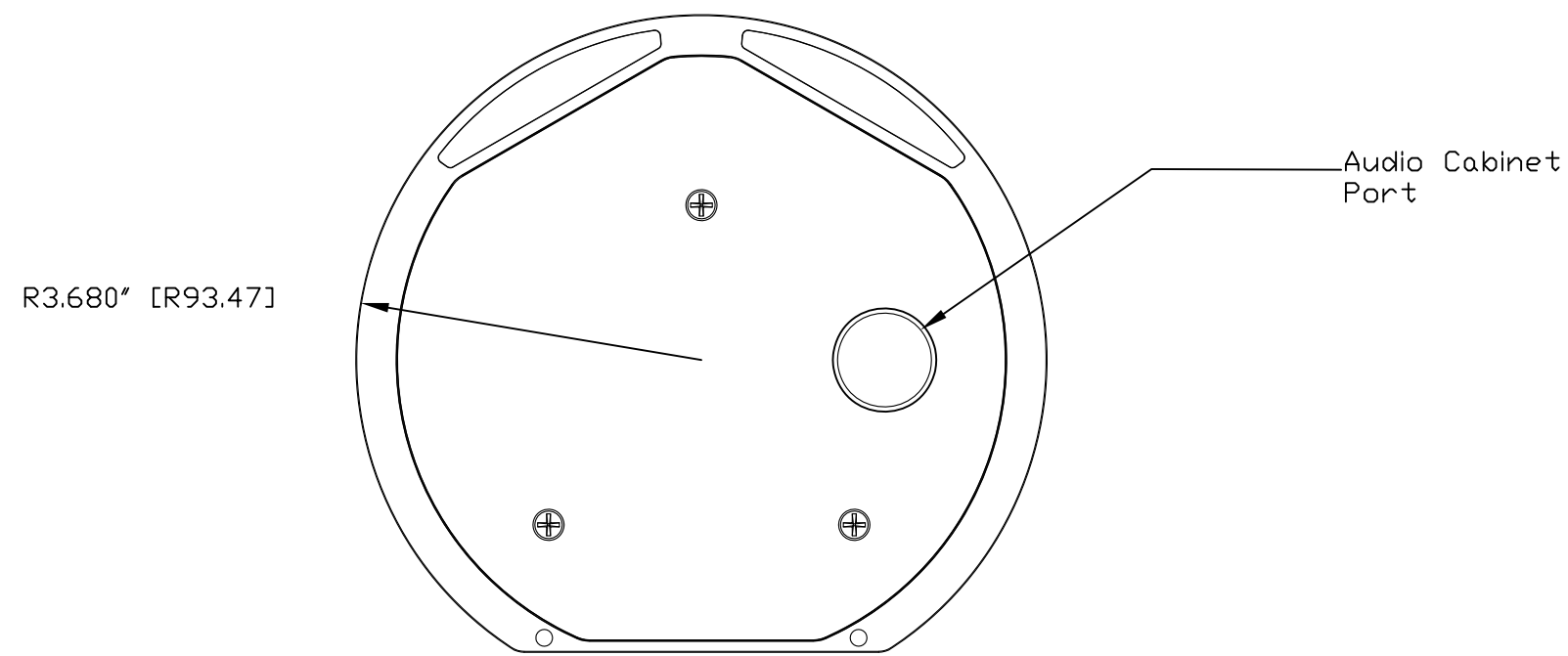
BOTTOM VIEW
