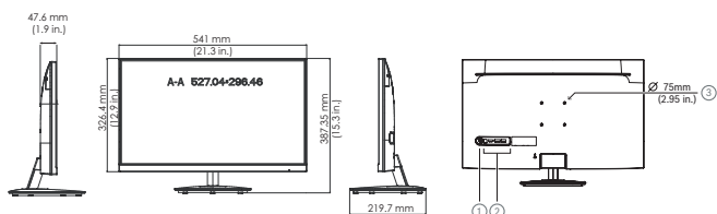
Fig. 1: Dimensions High Performance LED monitor (24 in.)
