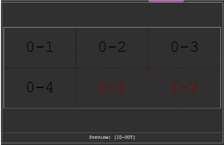
Figure 22: Video-wall Preview
