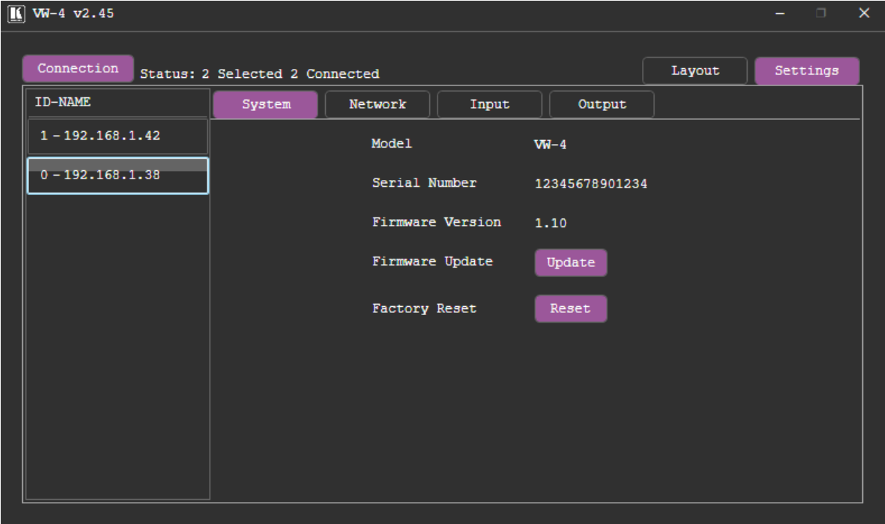
Figure 14: System Tab
